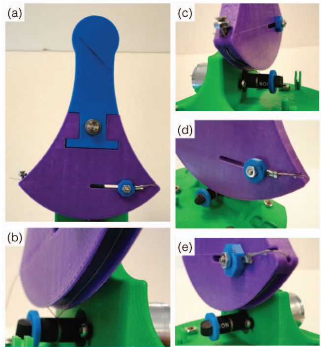
Fig. 5. Hapkit 3.0 Sector Pulley features: (a) Sector Pulley (b) Cable-Guide (c) Cable Attachment Screw (d) Pre-loading Feature (e) Cable-Routing Features.
