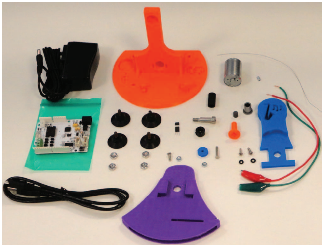
Fig. 4. Hapkit 3.0 assembly parts: Hapkit 3.0 is made from 3-D plastic structural material and readily available electronic and hardware components.
